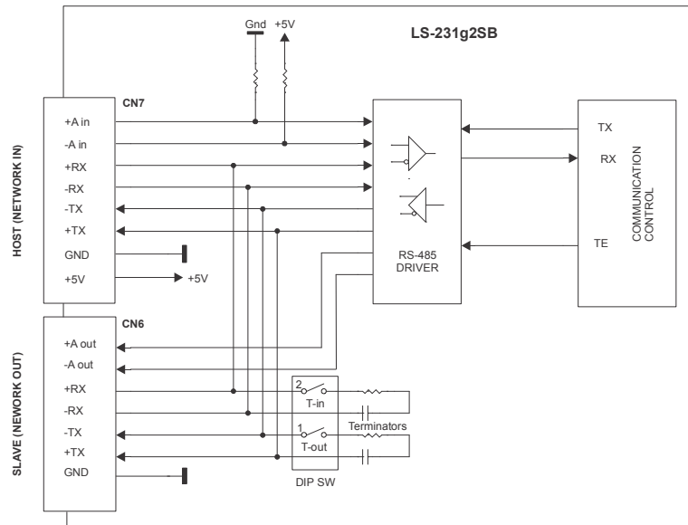
Communication interface
