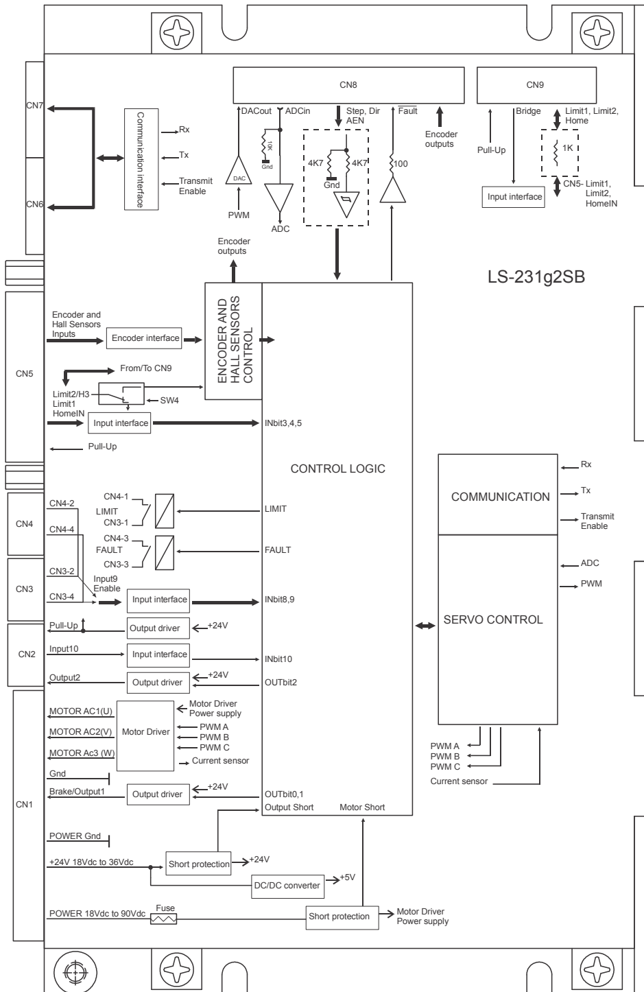
Block diagram
