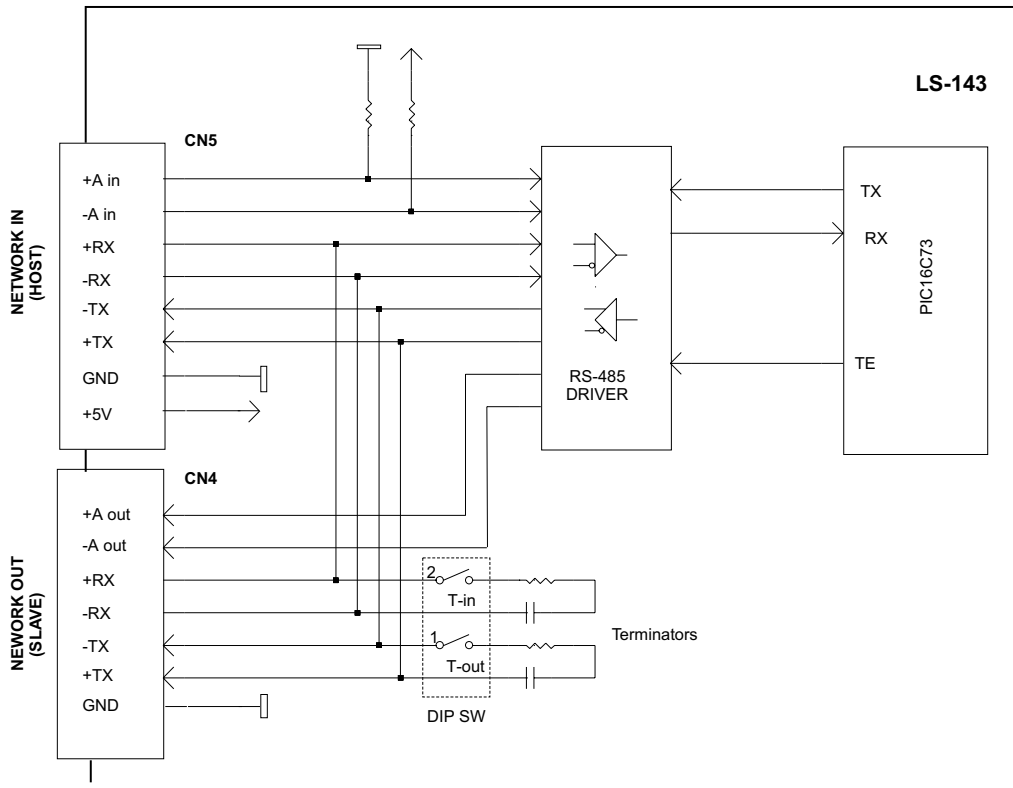
Stepper Drive Serial Interface
