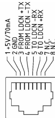
LDCN CONNECTOR FRONT VIEW
